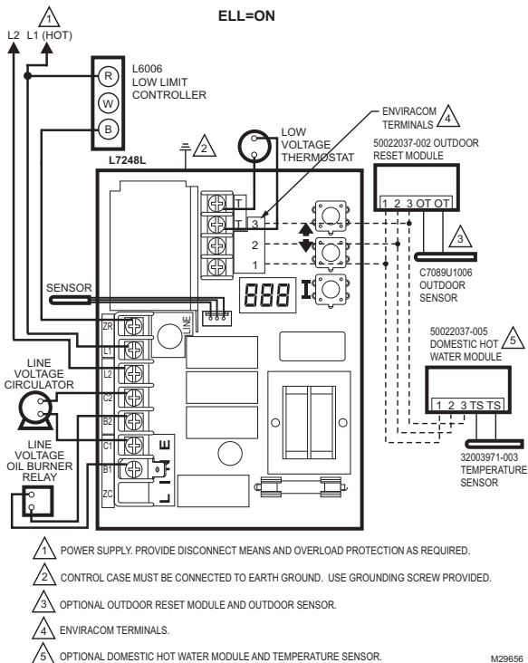
Fig. 13. L7248L External Low Limit connections.
