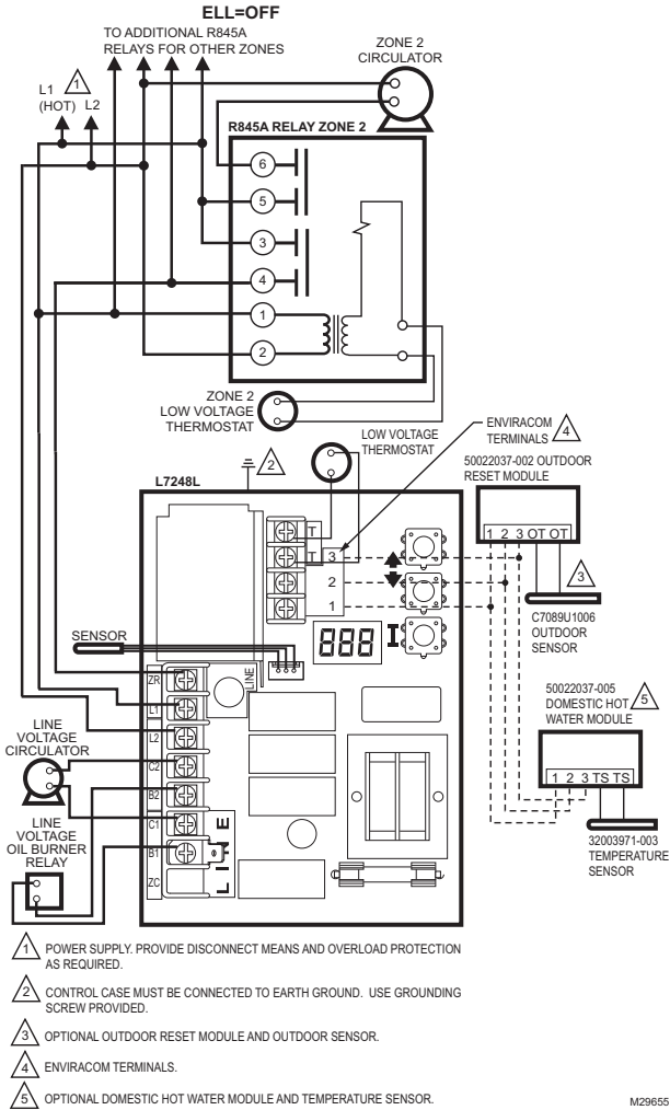
Fig. 12. L7248L multizone system with circulator connections.
