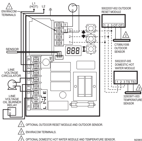
Fig. 9. L7224A,C; L7248A,C,L single zone connections.
