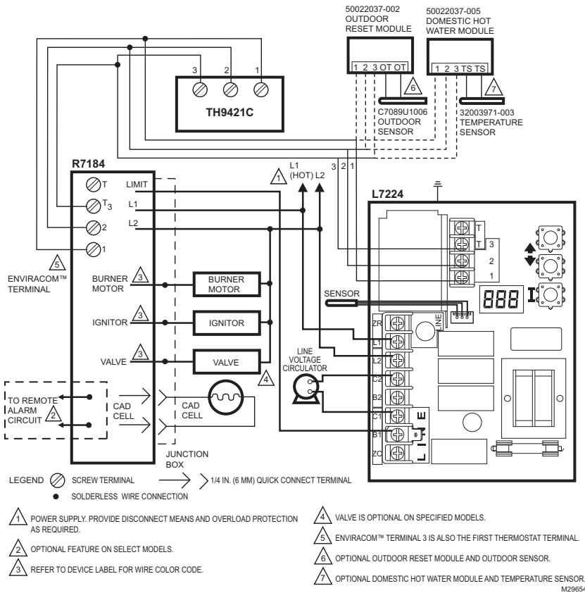
Fig. 11. L7224A,C multizone system with circulator connections and EnviraCOM™ thermostat.
