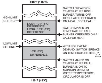
Fig. 8. Setpoints and differentials.
