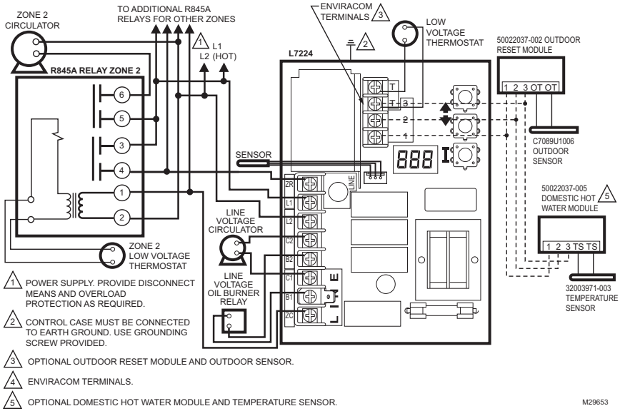
Fig. 10. L7224A,C multizone system with circulator connections.
